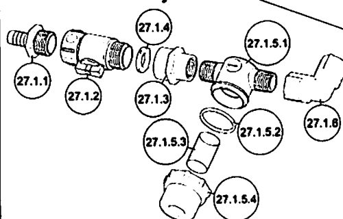
Intake Assembly
