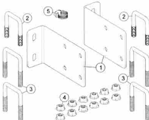
Boom Mount Kit (#5281303)
