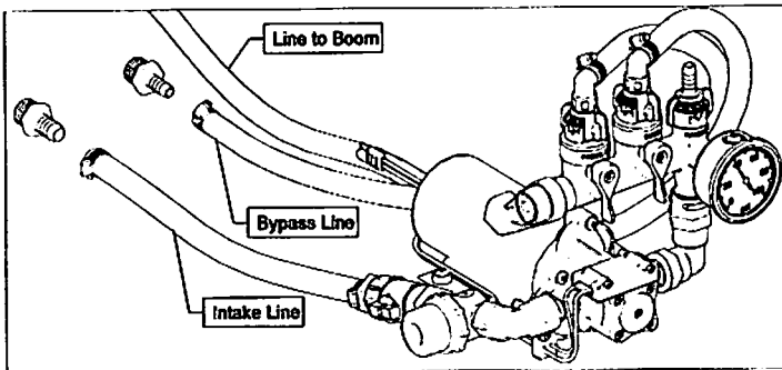
Manifold Detail
