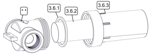
Strainer Detail
