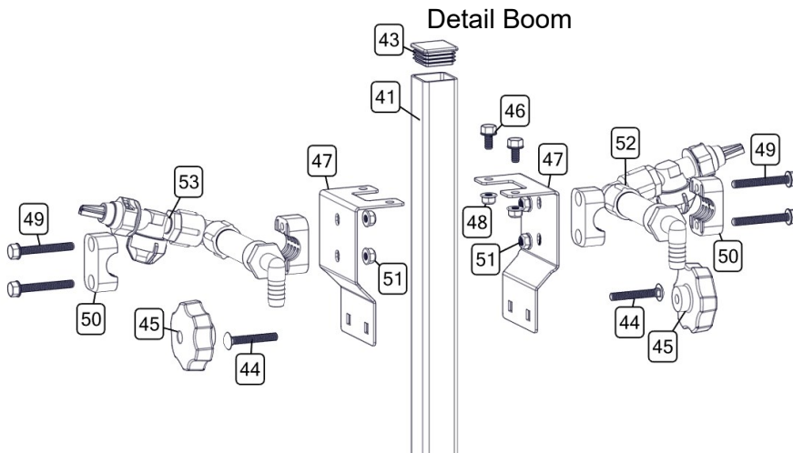
Broadcast Nozzle Assemblies
