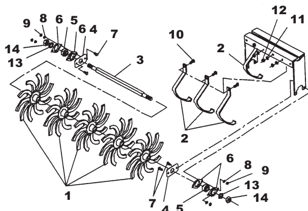
14-1/2" & 16" SPIDER WHEELS and COMPLETE GANGS
