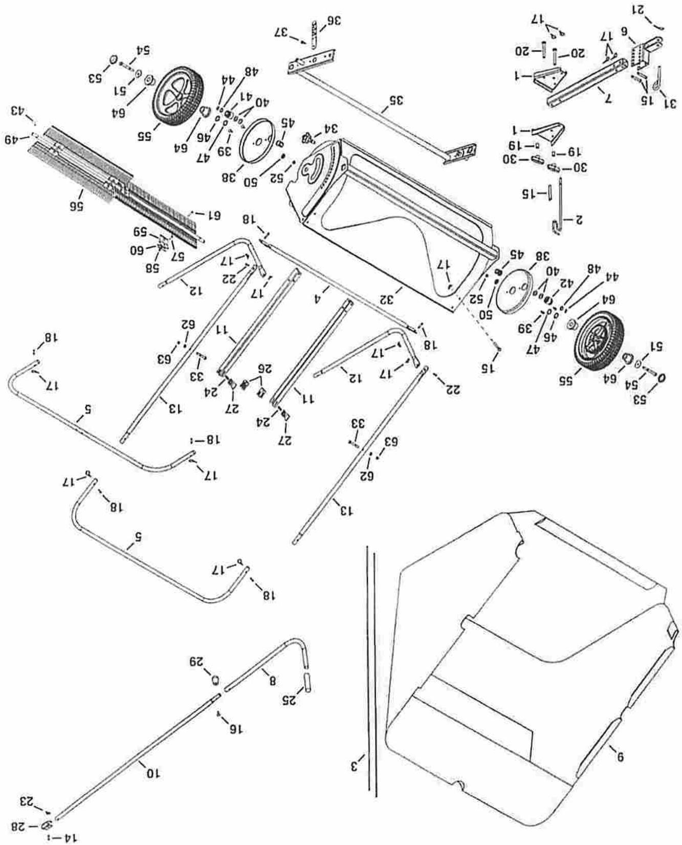
REPAIR PARTS ILLUSTRATION
